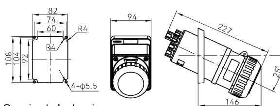
Opening hole drawing
