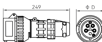
Plug (T)
