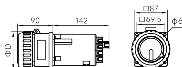
Socket without enclosure (M)
