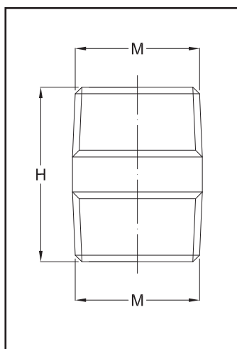
SELECTION TABLE OF ISO 7/1 SEALED NIPPLES
