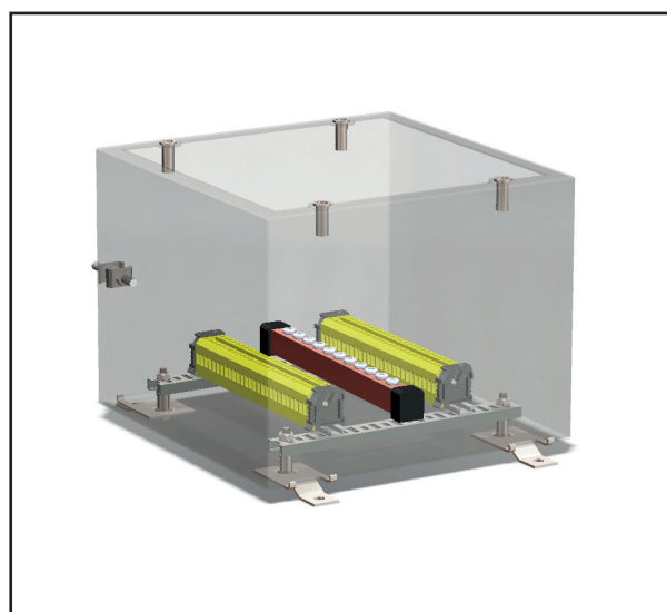
Example of feed-through terminal installation on top hat rail fastened to two pre-drilled mounting rails.
